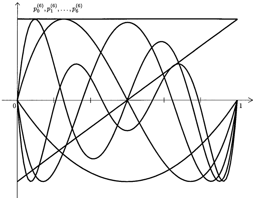
FIG. 1. The eigenfunctions p_k^{(6)}, k = 0, \dots, 6 for the Bernstein operator B_6 (scaled to have the same absolute maxima). Note the symmetries and the interlacing of the zeros.
