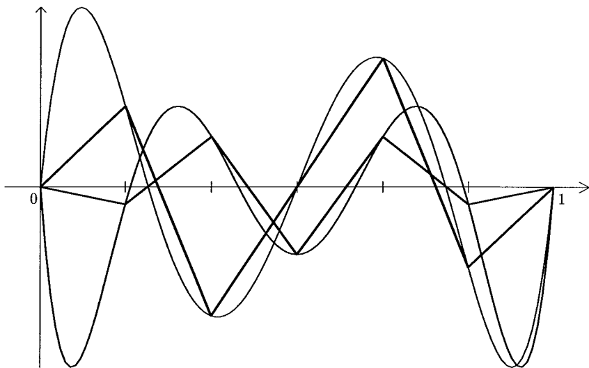
FIG. 2. The interlacing of the zeros of the piecewise linear interpolants to p_5^{(6)} , p_6^{(6)} .
